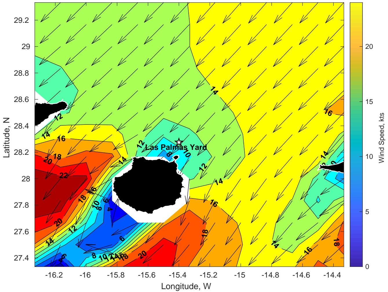
Winds (kts) for Las Palmas Yard at 04-May-2024 00:00:00
